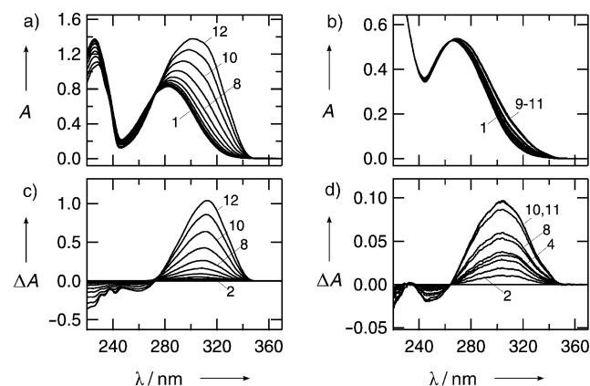
Figure 2. Progress of the photoreaction ( \lambda > 280 nm) of cis -1 at 80 K in 2-methylpentane glass (a and c) and in 2-methylpentane solvent at 273 K (b and d). Changes in the absorption curves versus time (0, 5, 10, 20, 40, 80, 160, 320, 640, 1280, 2560, and 5120 s for a; same intervals to 2560 s for b) and difference absorption bands ( A_t - A_0 ) for the 80 K (c) and 273 K (d) data are shown.
