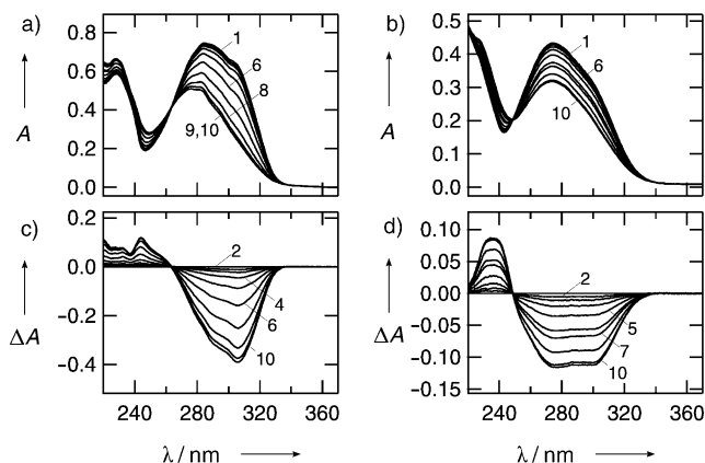
Figure 3. Progress of the photoreaction ( \lambda > 280 nm) of (E)-2 at 80 K in 2-methylpentane glass (a and c) and in 2-methylpentane solvent at 273 K (b and d). Changes in the absorption curves versus time (0, 5, 10, 20, 40, 80, 160, 320, 640, and 1280 s for a and b) and difference absorption bands ( A_t - A_0 ) for the 80 K (c) and 273 K (d) data are shown.
