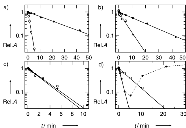
Figure 5. Changes in the absorbance maxima during irradiation of trans - 1 (a), cis - 1 (b), ( E )- 2 (c), and ( Z )- 2 (d) at 80 K in 2-methylpentane glass and 273 K in 2-methylpentane solution. The closed and open circles represent absorbance changes at 80 and 273 K, respectively.
