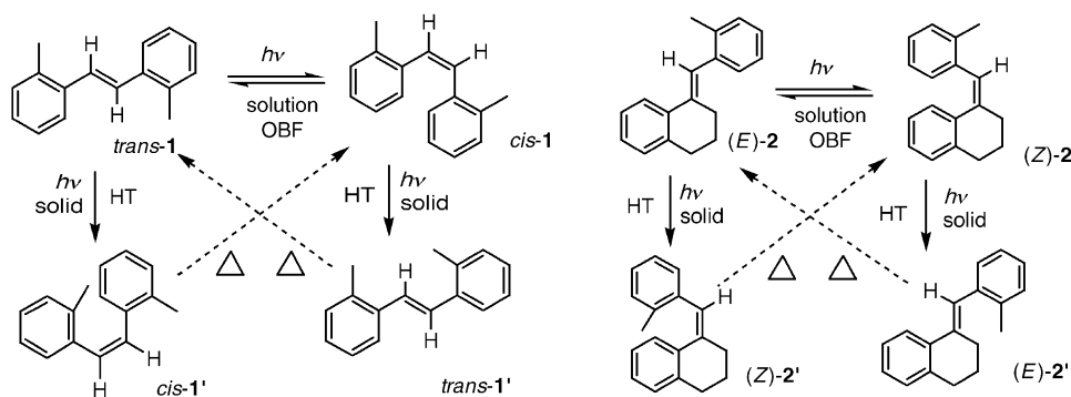
Scheme 2. Predicted photoisomerization pathways. Left: 2,2'-substituted stilbenes 1 ; right: ring-fused stilbene analogues 2 . Horizontal: photoisomerization in solution by OBF; vertical: isomerization in frozen solution by HT; diagonal: warming and thawing of the solid solution containing the HT product.
