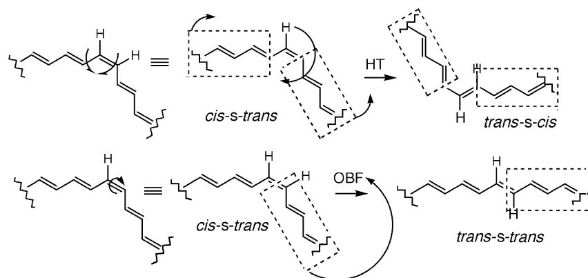
Scheme 1. Top: cis to trans isomerization by Hula twist (HT) with simultaneous conformational reorganization and one CH unit rotating out of the plane. Bottom: cis to trans isomerization by one-bond-flip (OBF) with half of the molecule rotating around a double bond.
